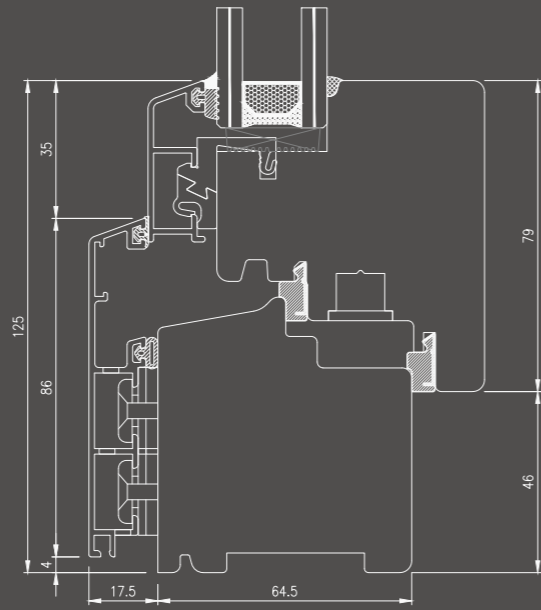
Standard Bottom Node - Window with Integrated Drip Cap
