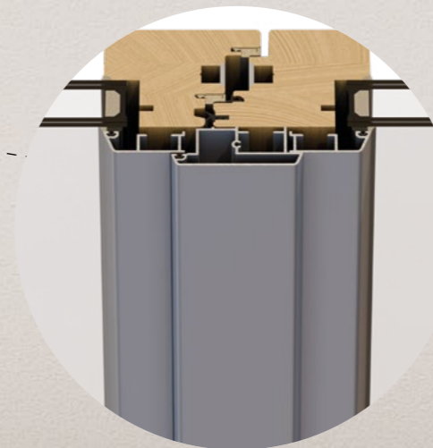
CENTRAL NODE ON THE EXTERIOR SIDE. AVAILABLE IN 3 VERSIONS.
