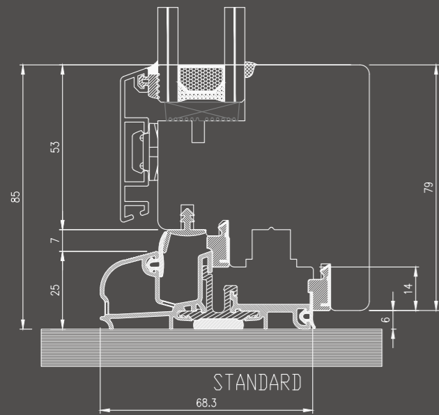
Bottom Node - French Door with Threshold
