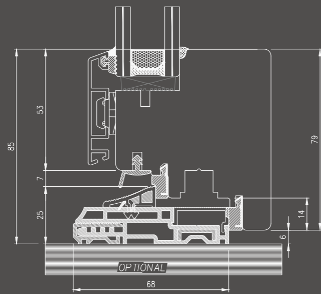
Bottom Node - French Door with Threshold
