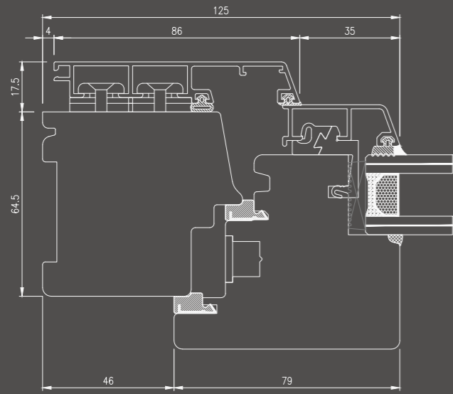
Top/Side Node - Window and French Door
