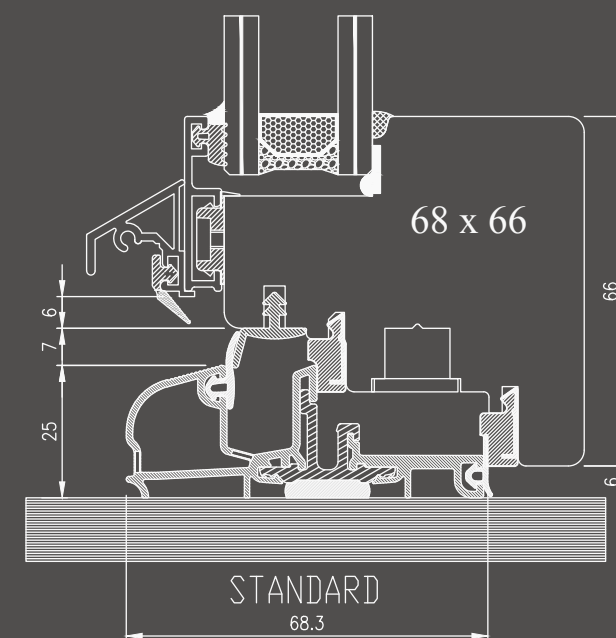
Bottom Mullion of french Door with Threshold
