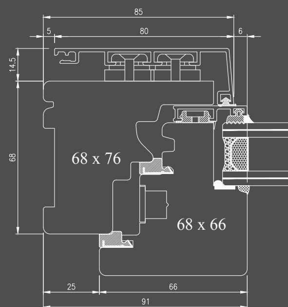
Upper/Side Node of Window and French Door
