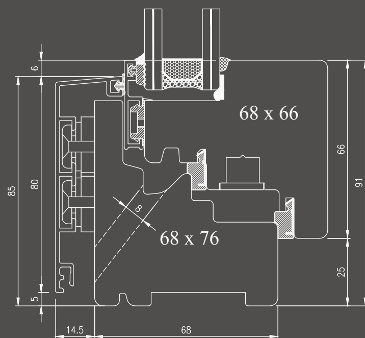
Bottom Mullion of Window
