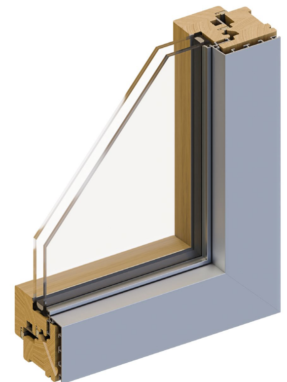
Window – Exterior Corner
