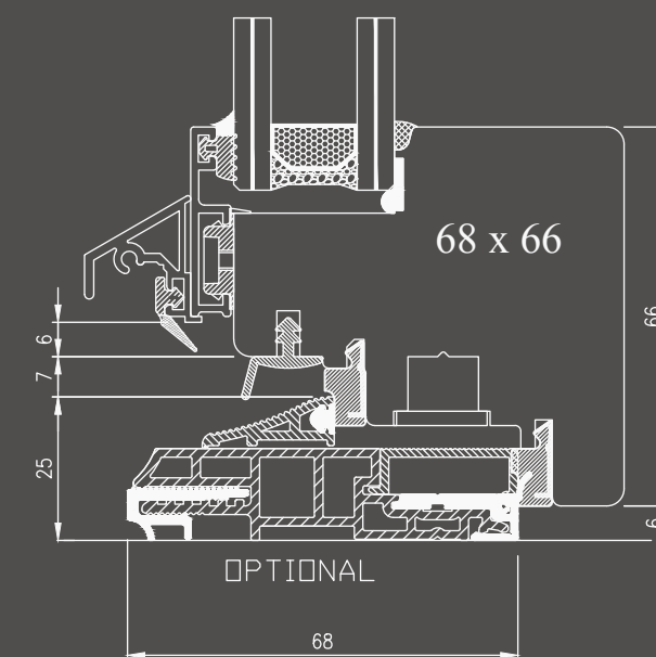
Bottom Mullion of french Door with Threshold
