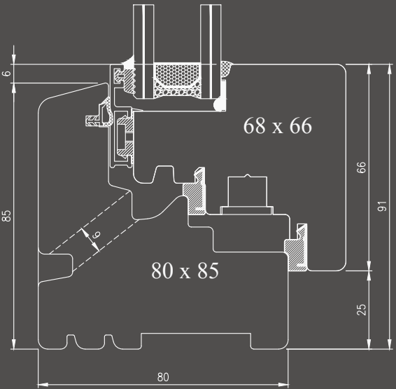
Bottom junction of window
