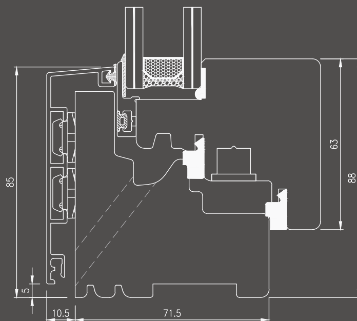
Window lower node
