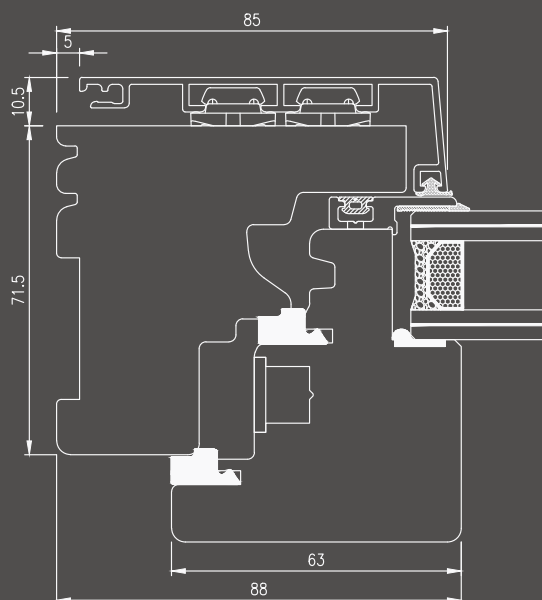
Upper/lateral node for windows and French windows
